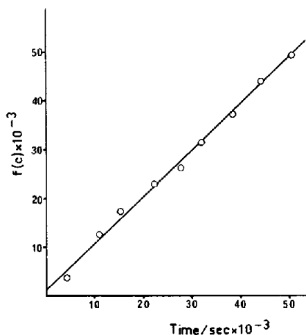
Fig. 2. Quantum yield determination at 343 nm of 2.7 Torr of 3-chloro-3-methyldiazirine plus 710 Torr of propane. Example of plots of the left-hand term f(c) of equation (see text) against time.
