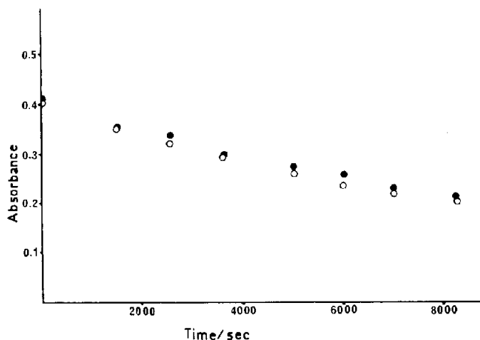
Fig. 5. Decay of two samples that absorb the same fraction of the incident light at 313 nm but contain different 3-chloro-3-methyldiazirine concentrations. The mercury lamp was used.
