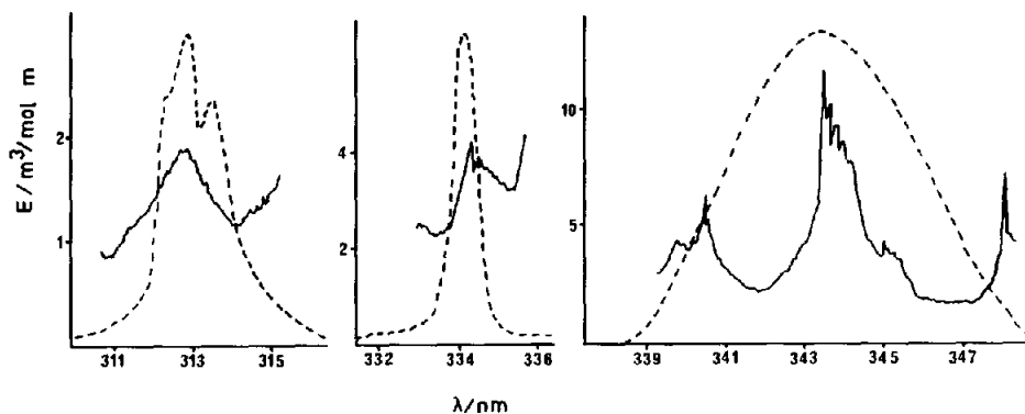
Fig. 1. The 3-chloro-3-methyldiazirine bands irradiated (—) and the photolysis light (-----) in arbitrary units.
