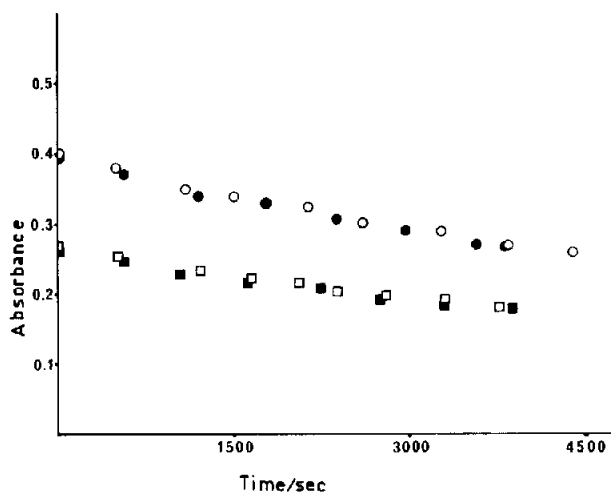
Fig. 4. Decay of two samples of 3-chloro-3-methyldiazirine that absorb the same fraction of the incident light: ○, ●, runs at 334 and □, ■, at 343 nm. The filled symbols indicate the sample pressurized with 710 Torr of propane. The xenon lamp was used.
