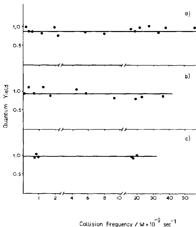
Fig. 3. Quantum yield of 3-chloro-3-methyldiazirine decomposition vs. collision frequency at (a) 313 nm, (b) 334 nm and (c) 343 nm.
